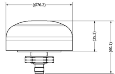
GNSS-L125-PSTNC
